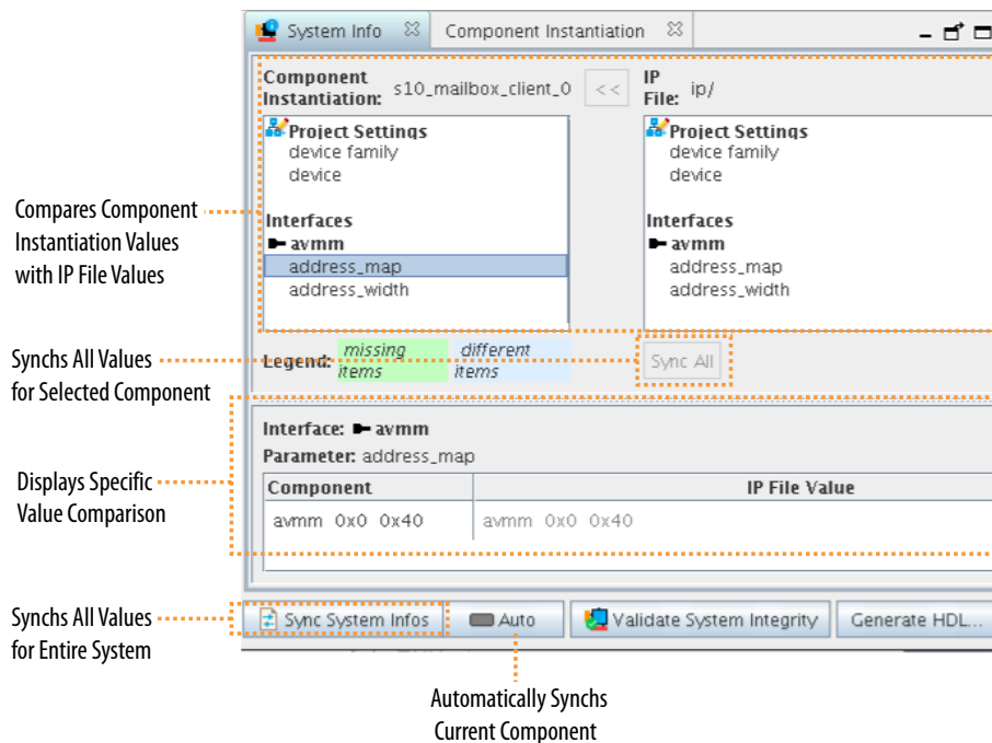
Figure 78. System Info Tab
