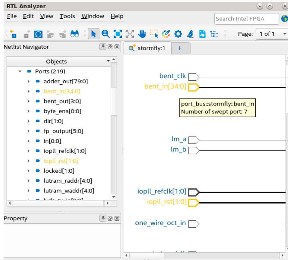
Figure 14. Sweep Hints View in the RTL Analyzer
