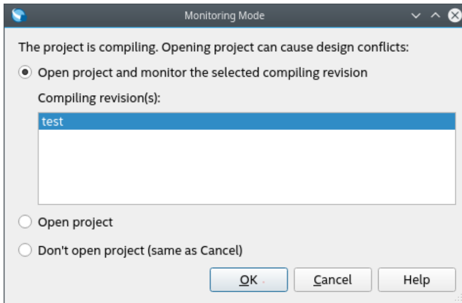
Figure 117. Monitoring Mode
