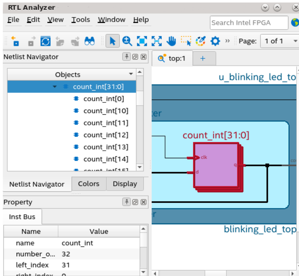
Figure 32. Bundled Instance
