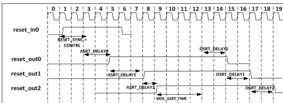
Figure 236. Basic Sequencing
