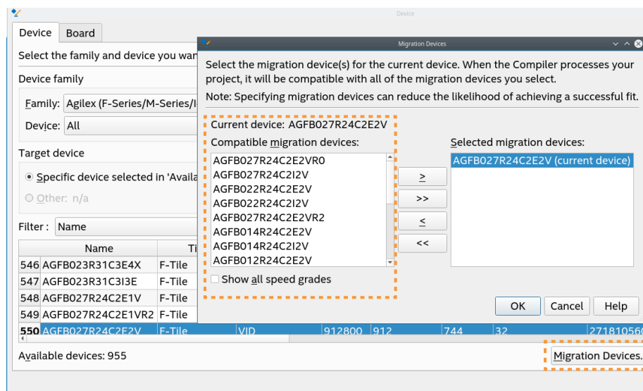
Figure 1. Devices Available for Migration from Selected Device
