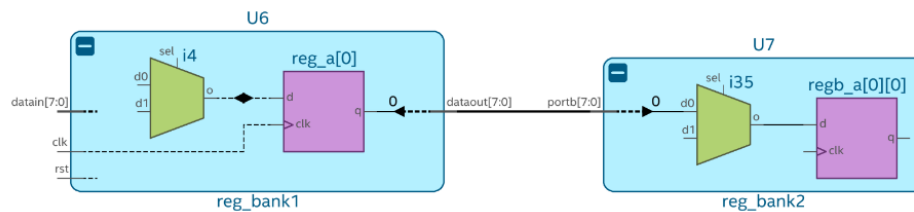
Figure 61. Targeting Pins in Cells Example
