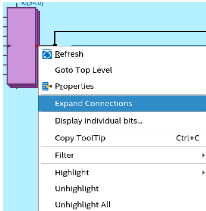
Figure 40. Expand Connections
