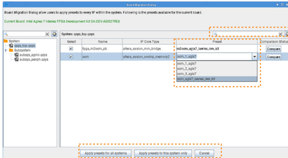
Figure 59. Setup Comparisons
