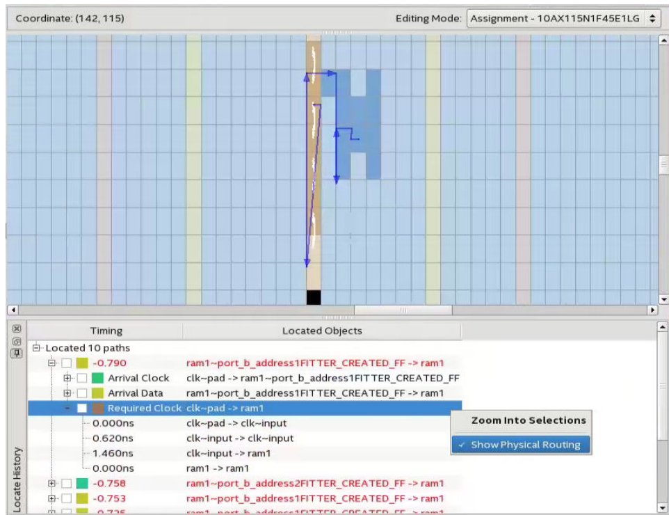
Figure 104. Highlight Routing
