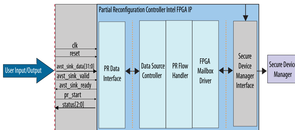
Figure 11. Partial Reconfiguration Controller (Avalon Streaming Interface)
