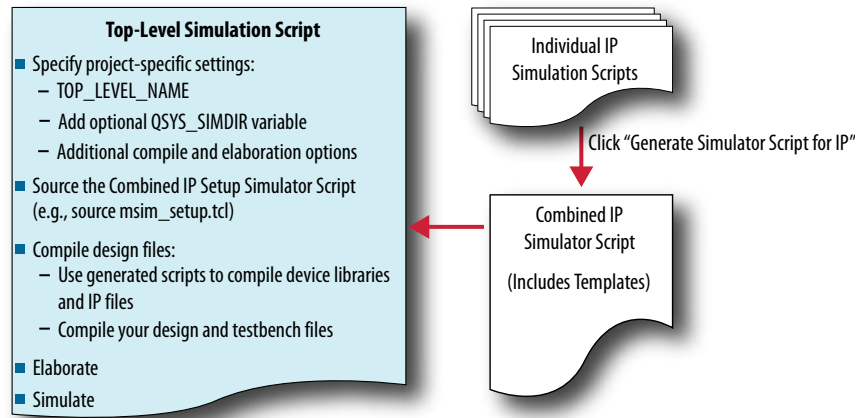
Figure 41. Incorporating Generated Simulator Setup Scripts into a Top-Level Simulation Script
