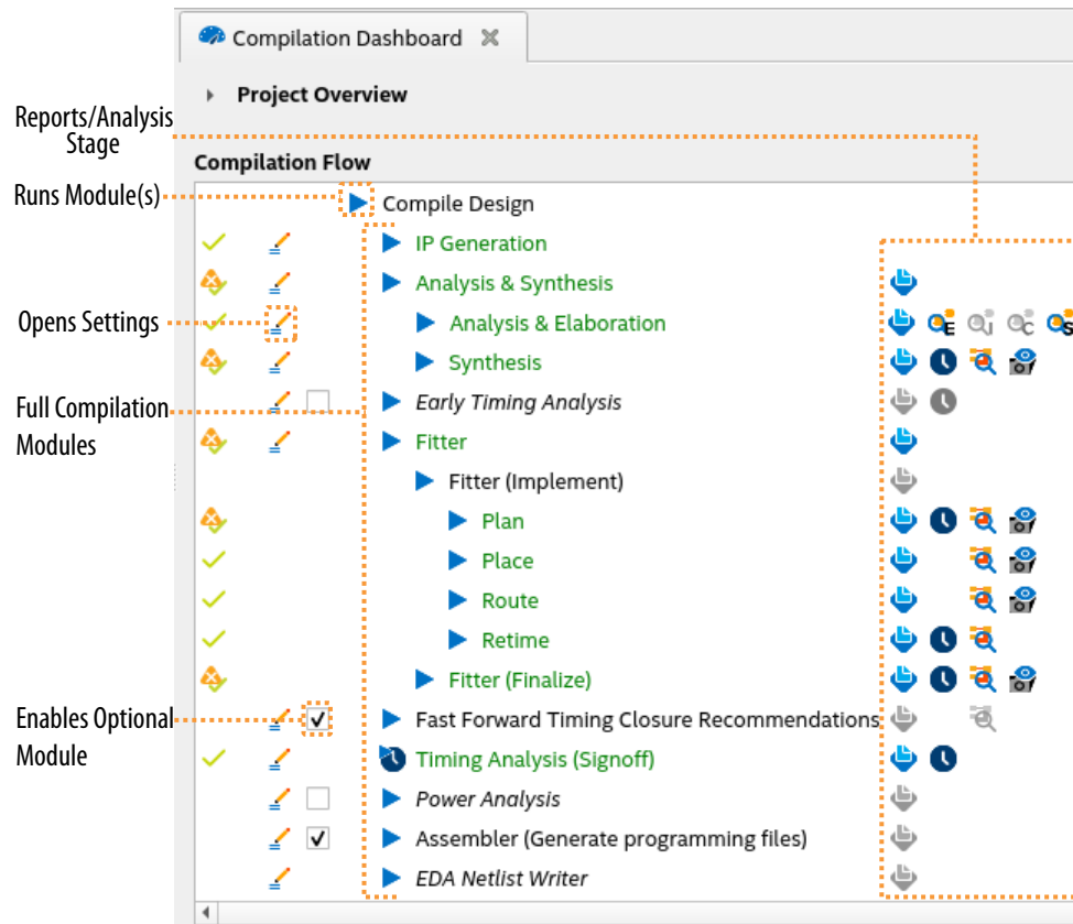
Figure 1. Compilation Dashboard
