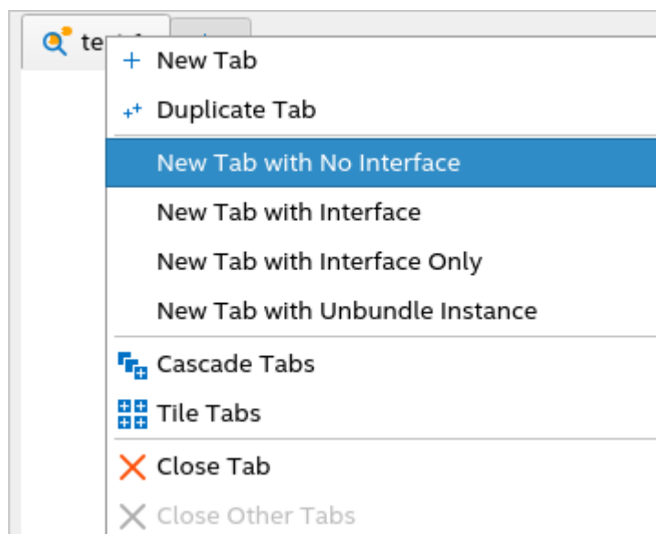
Figure 27. Interface Modes
